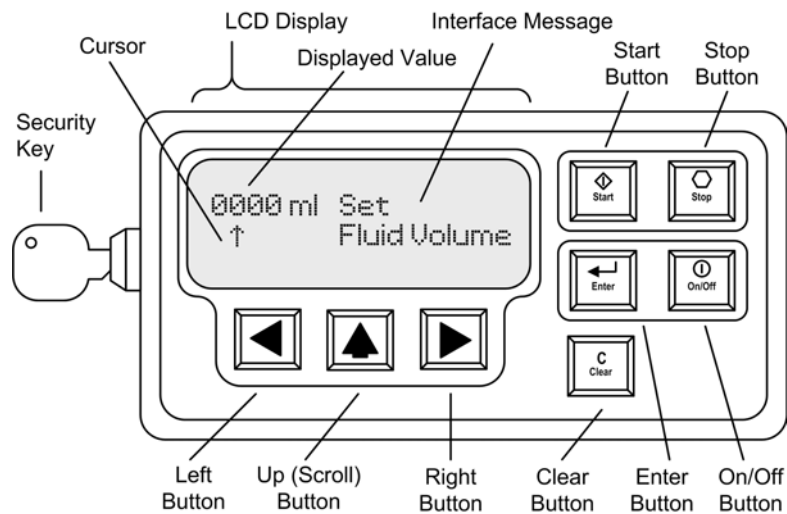
Figure 2: A simplified representation of the Baxter Ipump's human-device interface. Note that the actual pump contains additional controls and information conveyances.
